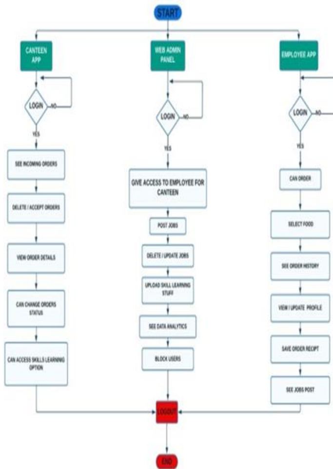
Figure 3: Flow chart of Canteen Application.
