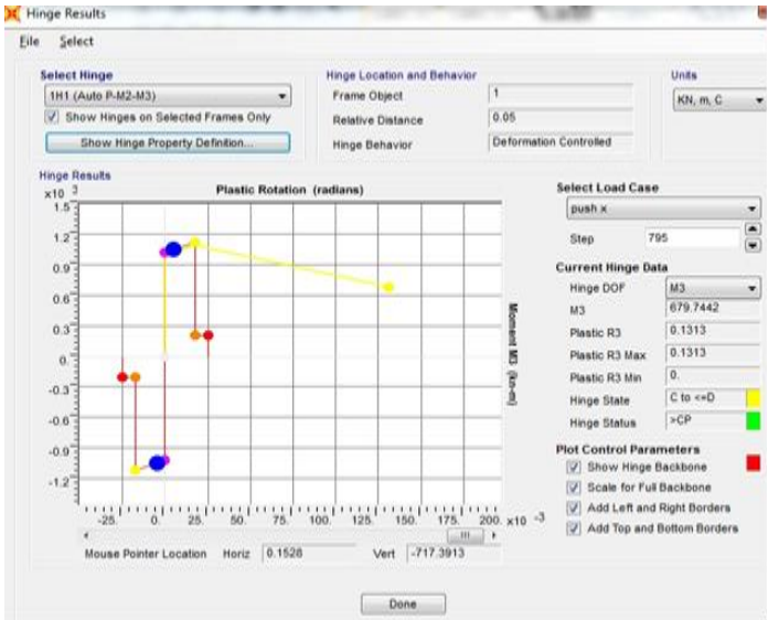
Figure 10: Acceptance criteria for Column (M3).
