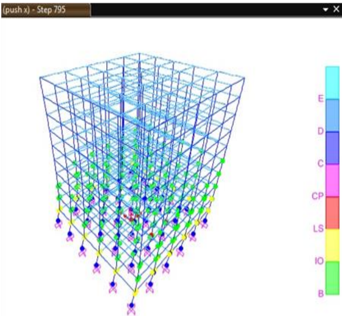
Figure 9: Deformed Shape.
