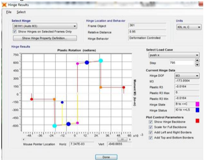
Figure 11: Acceptance criteria for Beam (M3).
