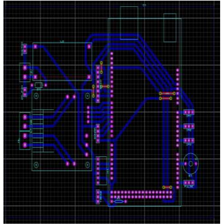
Figure 10: PCB layout.
