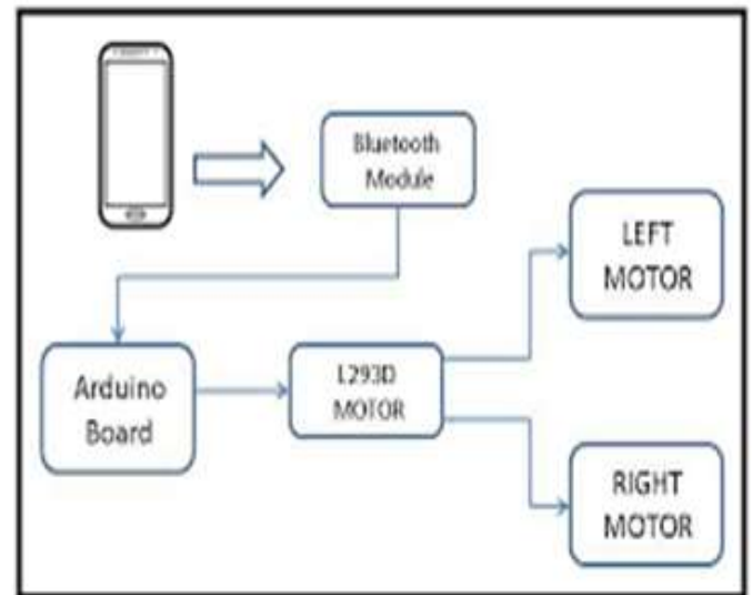
Figure 11: Flowchart implementation.
