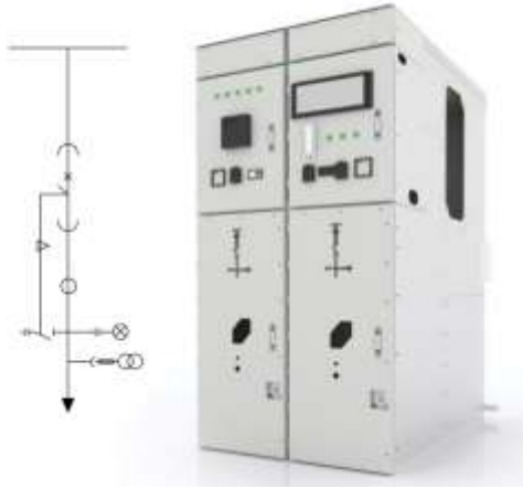
Figure 7: IF/OF SLD with Panel
