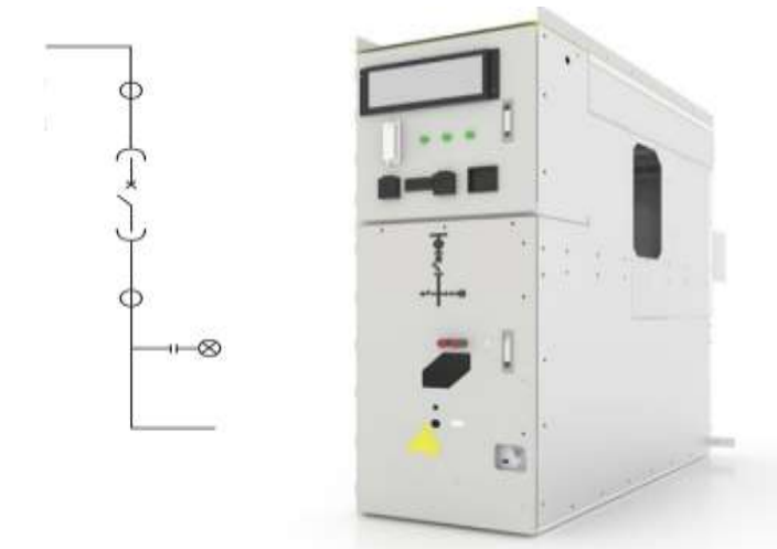
Figure 8: Busbar compartment.
