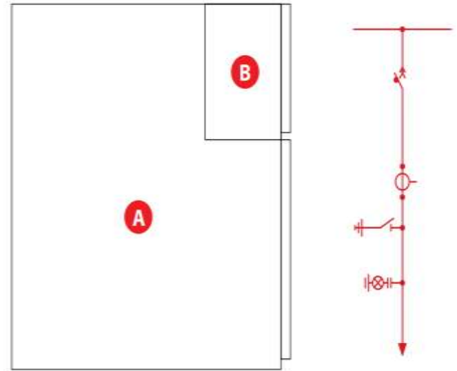
Figure 1: Secondary compartment.
